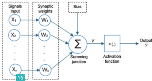
Fig. 1. The structure of the neural network unit
