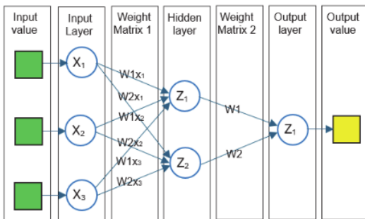
Fig. 2. Multilayer artificial neural network
